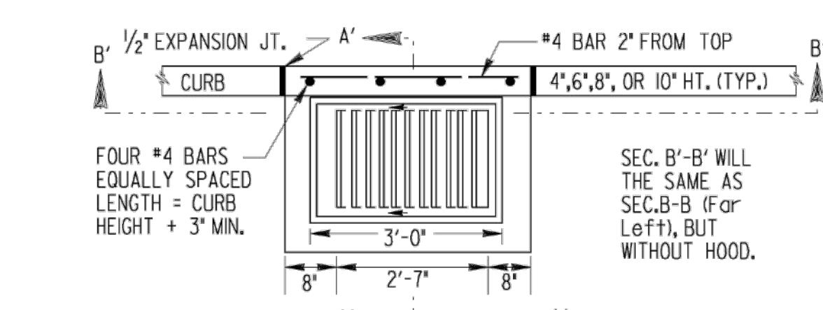
PLAN VIEW SCALE: 1/2" = 1 FT.
