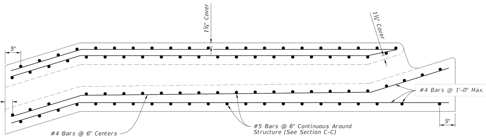
SIDE ELEVATION
