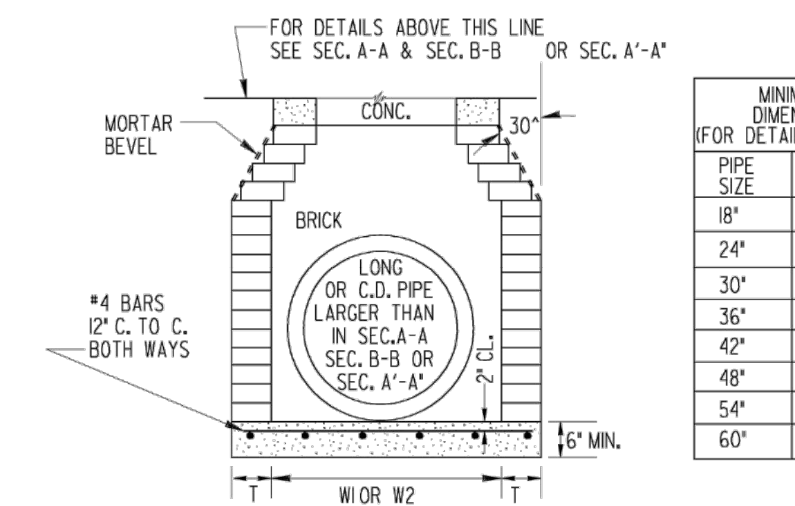
ALTERNATE-REDUCTION OF W1 OR W2 DIMENSIONS WITH BRICK MASONRY SCALE: 1/2" = 1 FT.
