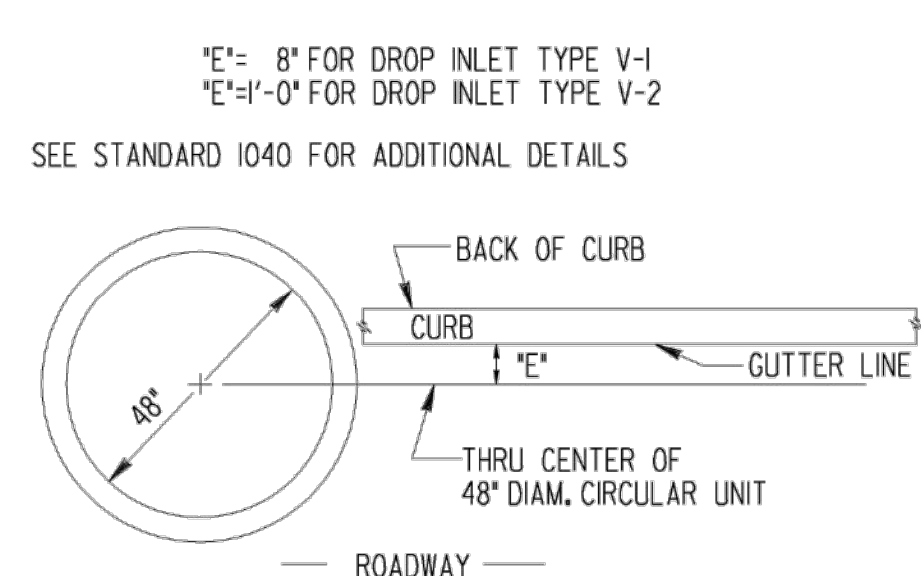
ALTERNATE - STANDARD IO40 CIRCULAR SECTIONS - PLAN VIEW LOCATION. NO SCALE
