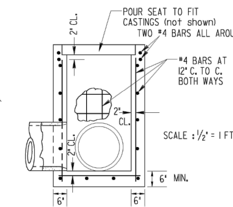
ALTERNATE- CAST-IN-PLACE REINFORCED CONCRETE
