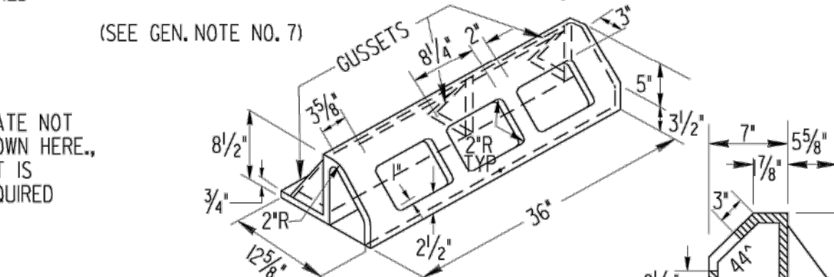
DETAIL OF HOOD (mountable) (use with Tp7 Curb)
