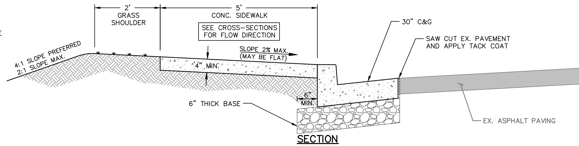
SECTION
