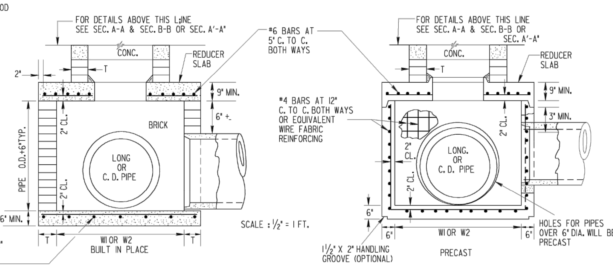
DETAIL OF REDUCING W1 OR W2 DIMENSIONS WITH REDUCER SLAB.
