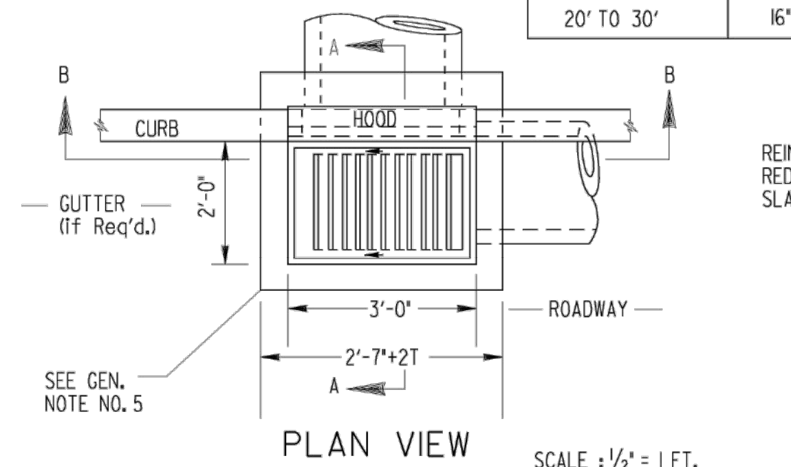
PLAN VIEW SCALE: 1/2" = 1 FT.
