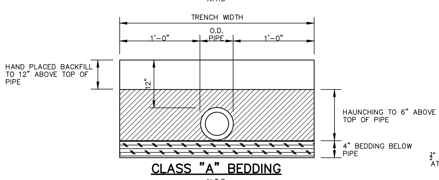
TYPICAL BEDDING REQUIREMENTS
