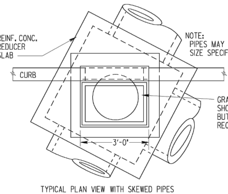
TYPICAL PLAN VIEW WITH SKEWED PIPES
