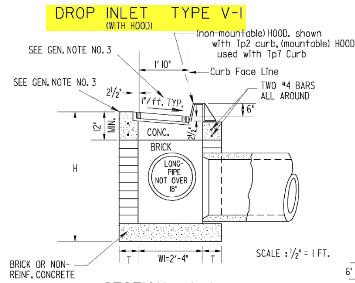
SECTION A-A (SEE GEN. NOTE NO. 7)
