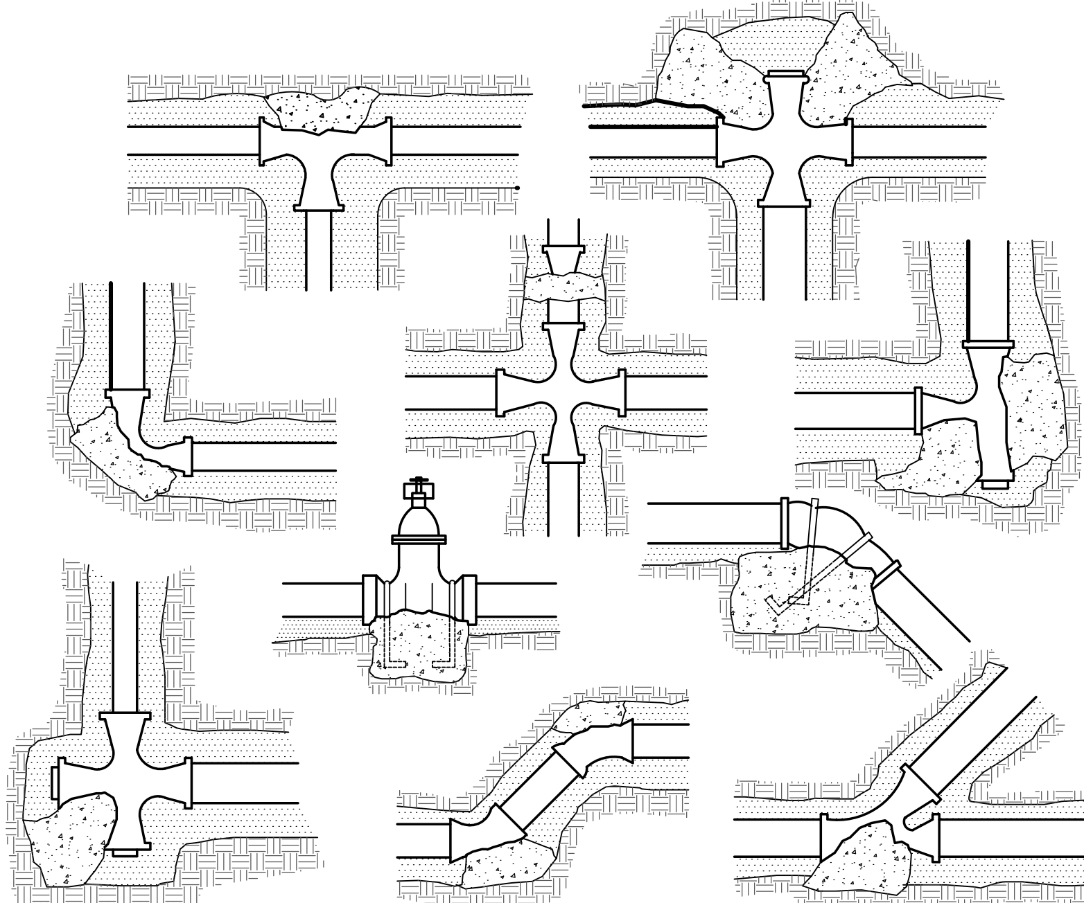
TYPICAL THRUST BLOCKS LOCATIONS DETAIL N.T.S.
